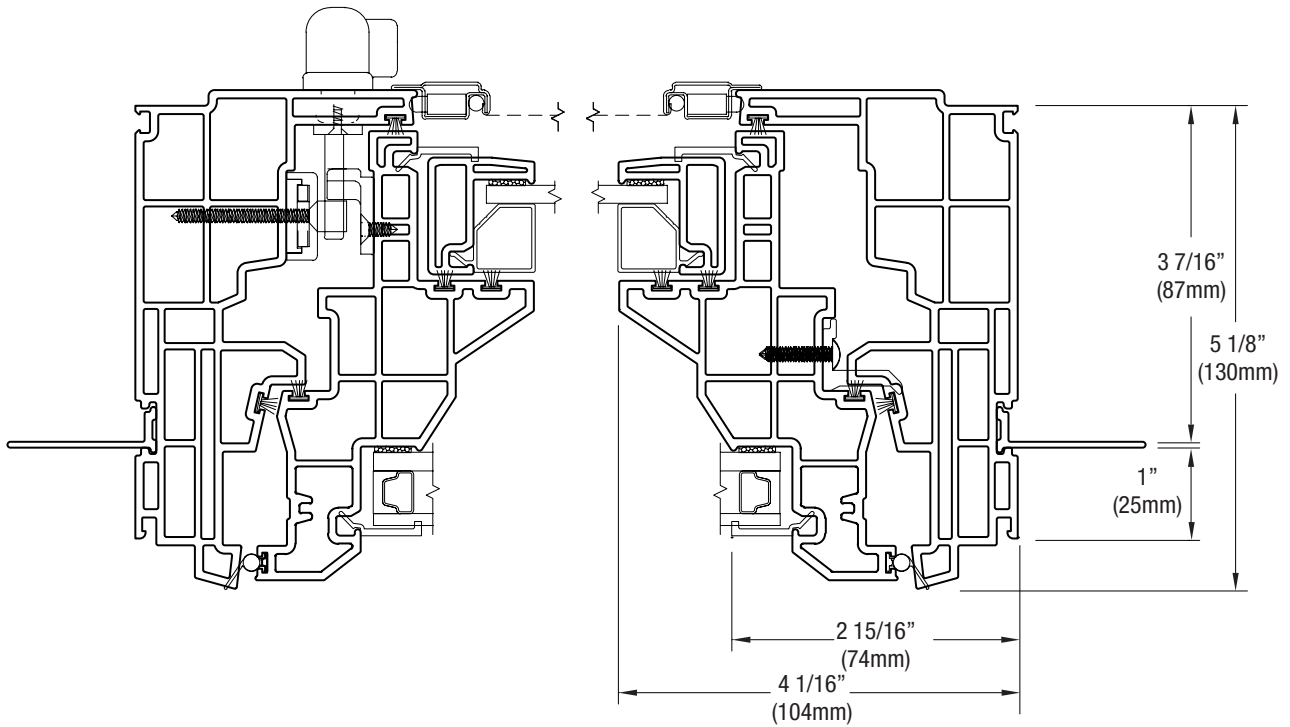
Horizontal View
